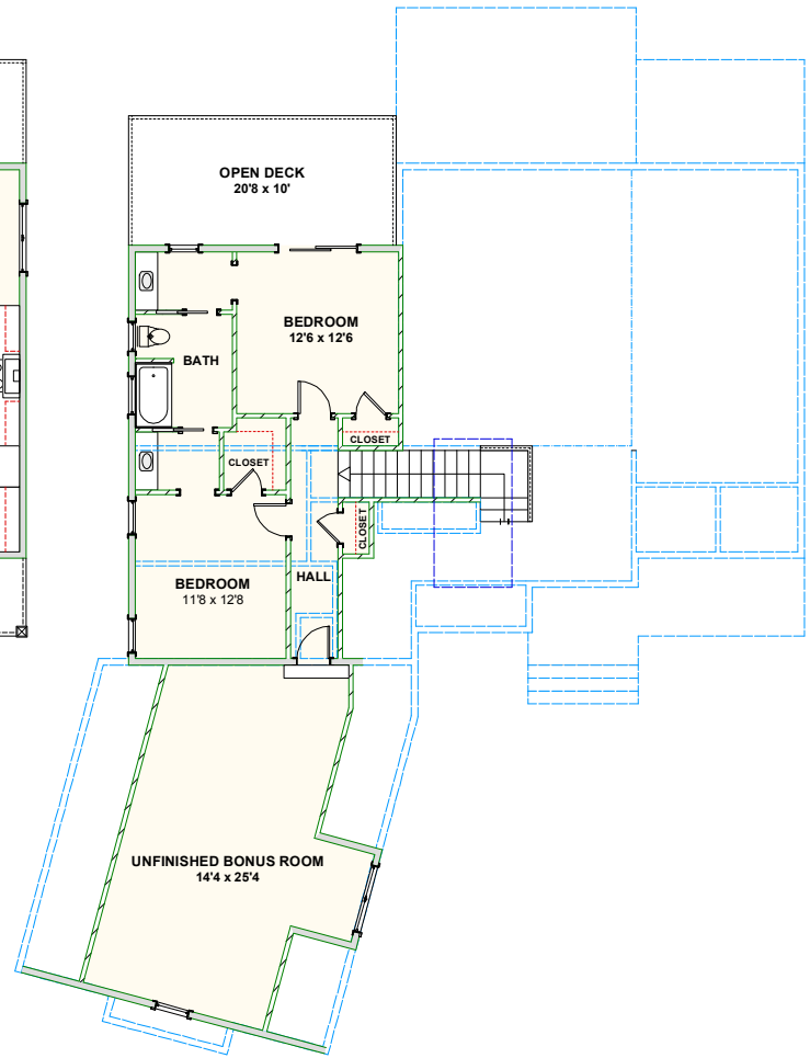
2ND FLOOR - FLOOR PLAN
